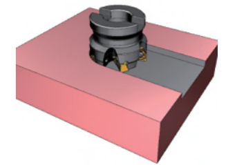
Slot milling
