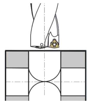
3. Cross-hole drilling
