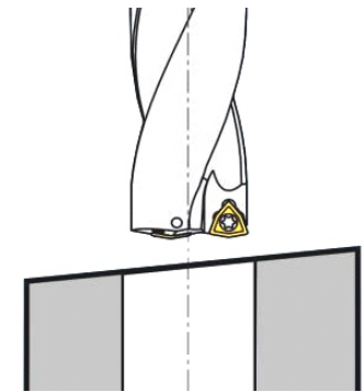
2. Drilling on inclined surface
