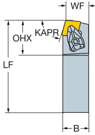
DCBNR/L 75.0°
