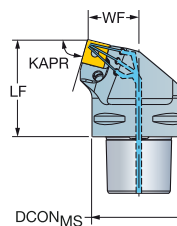
Cx-PSRNR/L..HP 75.0°
