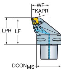
Cx-PSKNR/L..HP 75.0°
