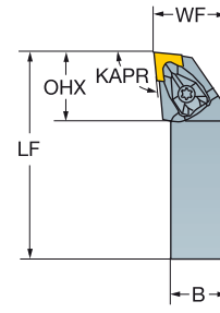
DCLNR/L 95.0°
