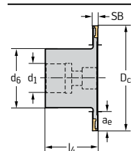
Shell mill mount DIN 138 transverse keyway
