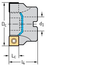
Shell mill mount DIN 138 transverse keyway
