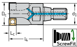
ScrewFit
