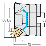
Shell mill mount DIN 138 transverse keyway
